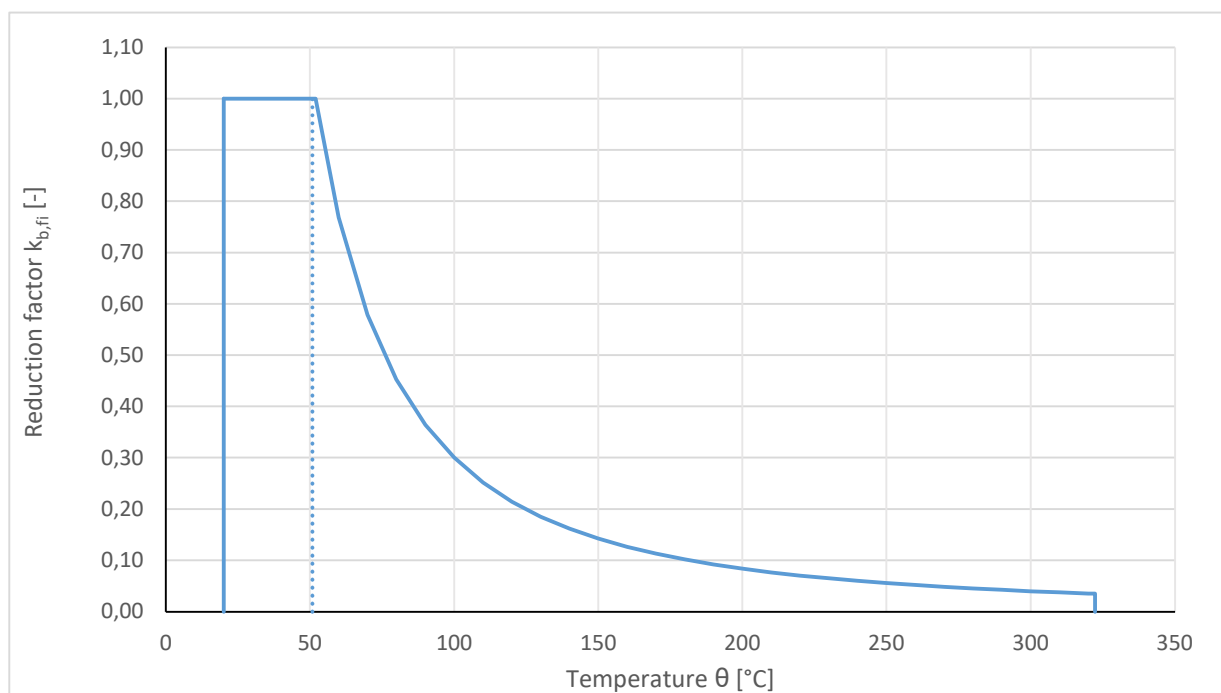
Figure C1: Example of the graph of reduction factor k_{fi}(\theta) for concrete strength class C20/25 for good bond conditions
